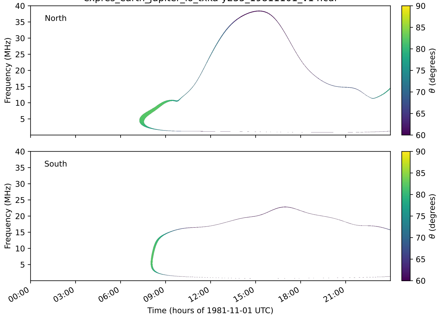
expres_earth_jupiter_io_txka-y235_19811101_v14.cdf
