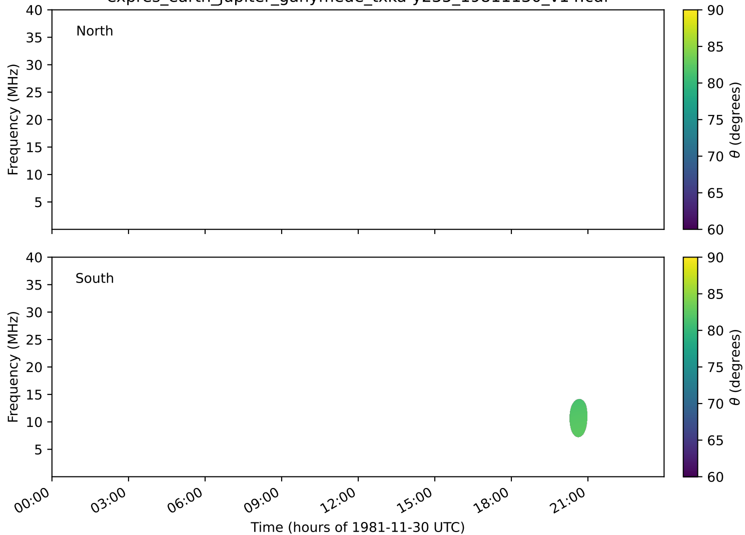
expres_earth_jupiter_ganymede_txka-y235_19811130_v14.cdf
