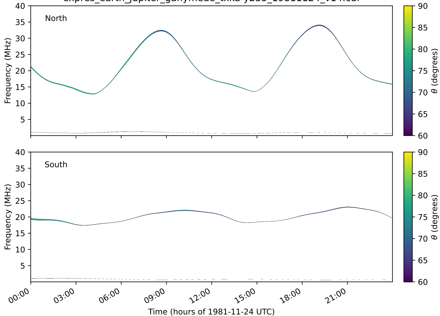
expres_earth_jupiter_ganymede_txka-y235_19811124_v14.cdf
