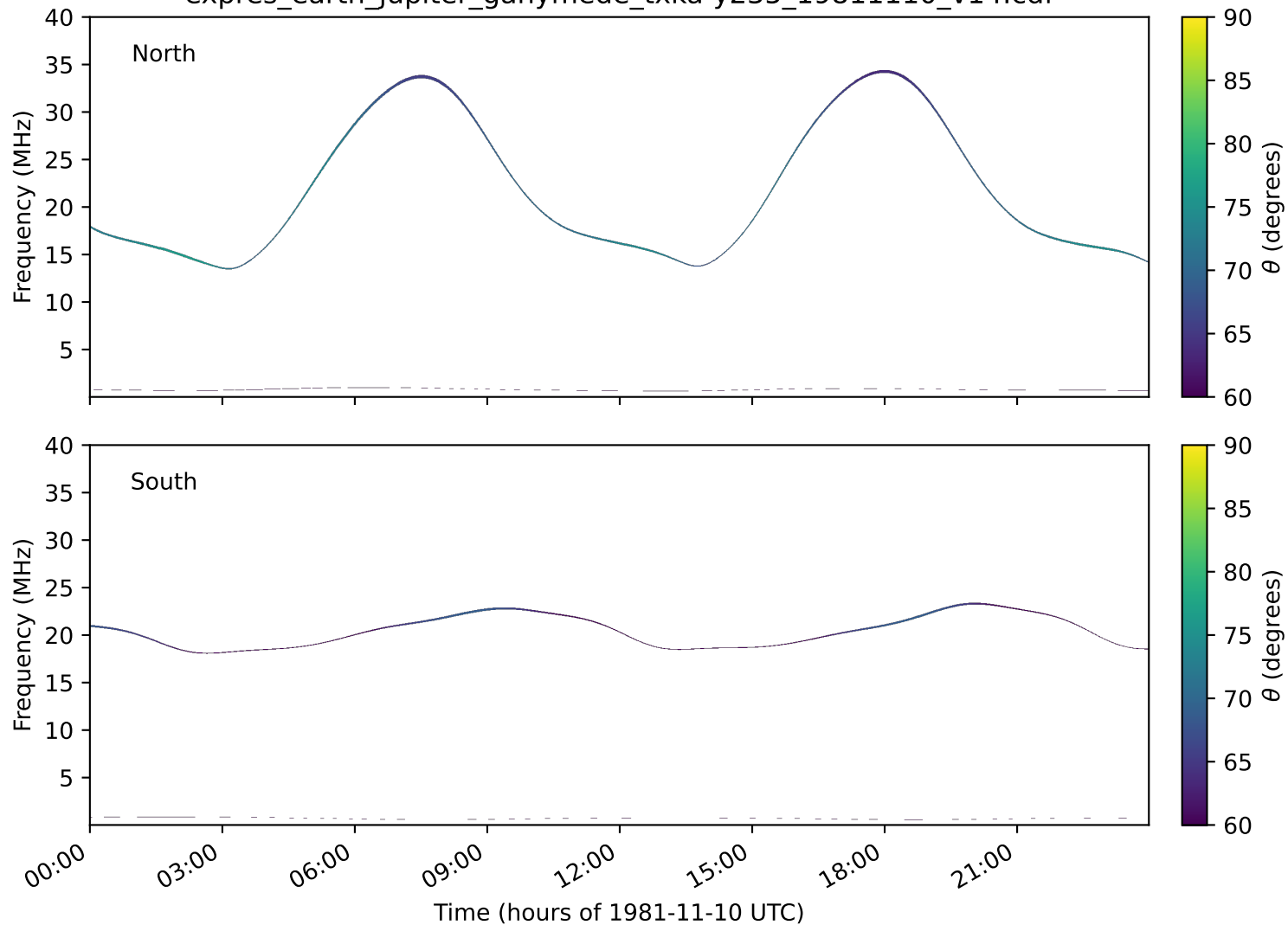
expres_earth_jupiter_ganymede_txka-y235_19811110_v14.cdf
