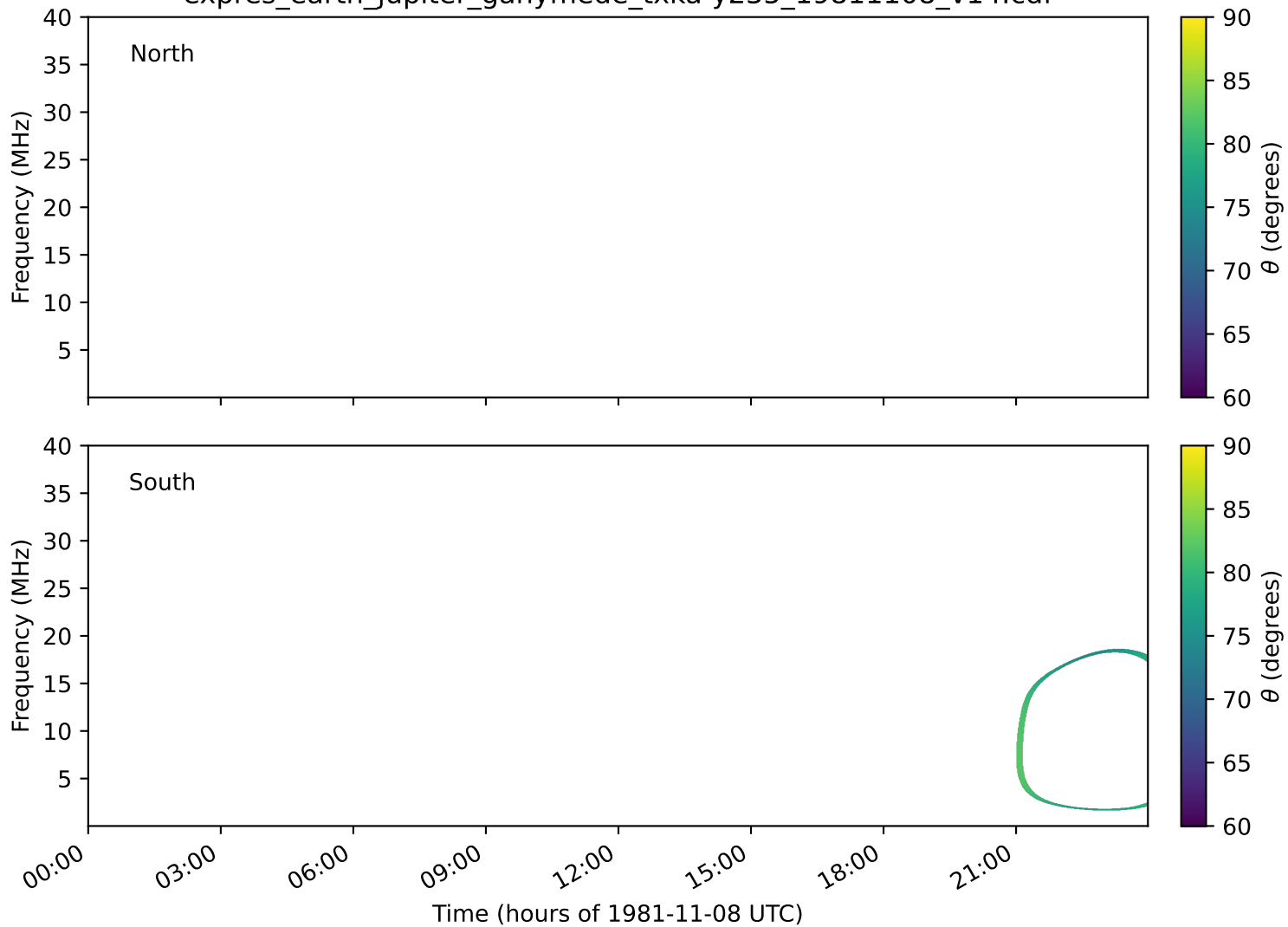
expres_earth_jupiter_ganymede_txka-y235_19811108_v14.cdf
