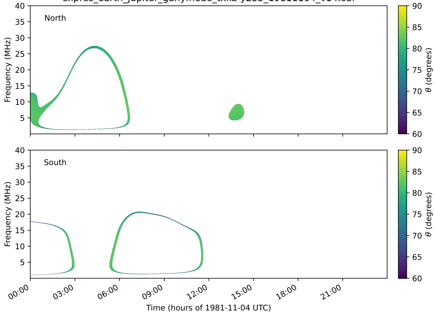
expres_earth_jupiter_ganymede_txka-y235_19811104_v14.cdf
