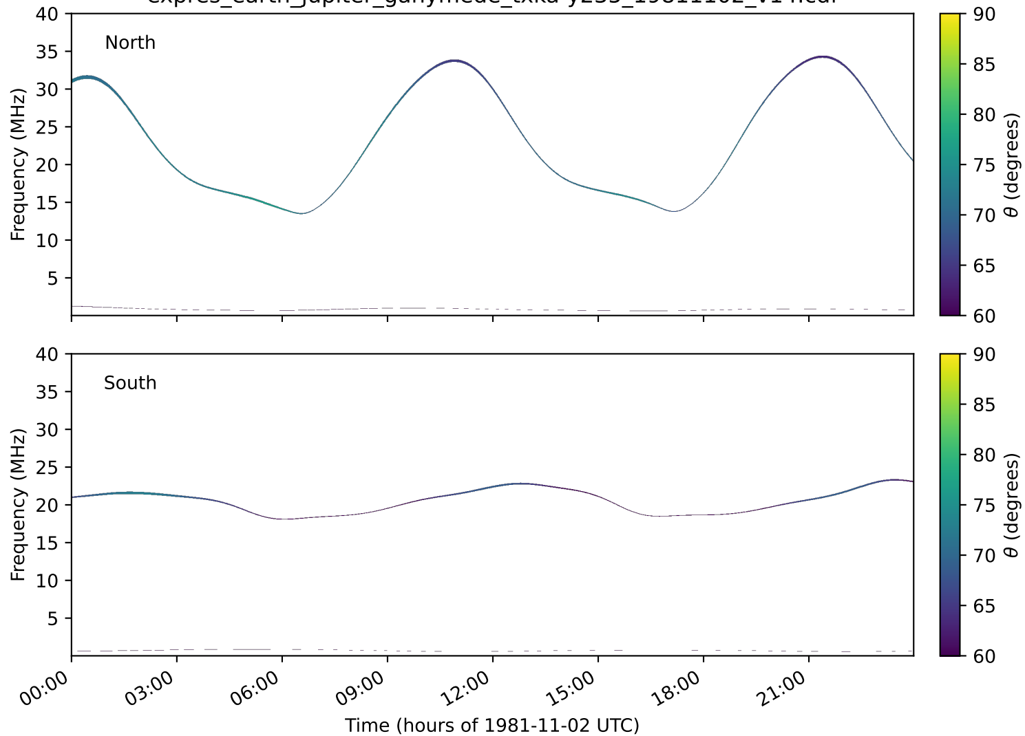
expres_earth_jupiter_ganymede_txka-y235_19811102_v14.cdf
