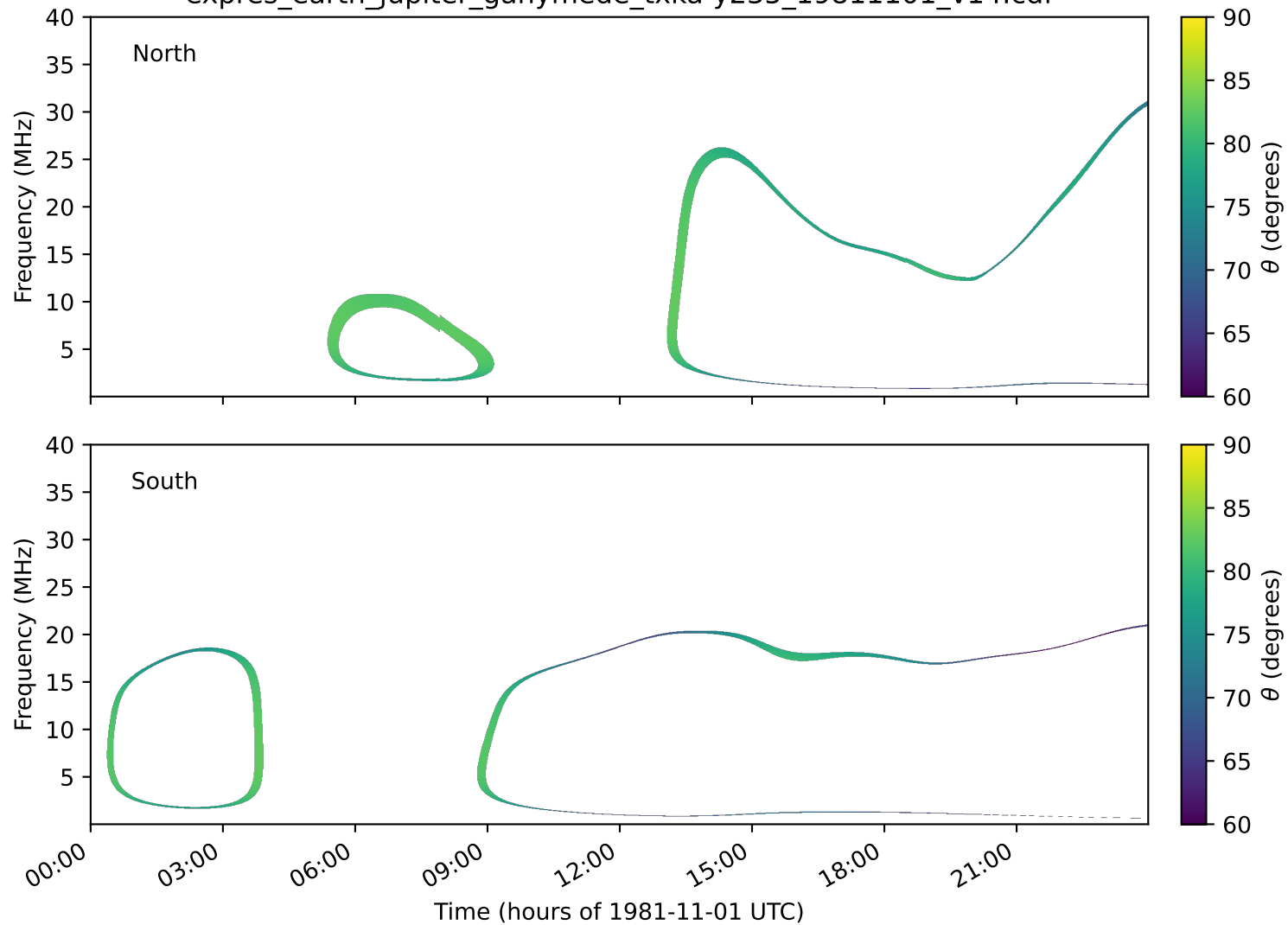
expres_earth_jupiter_ganymede_txka-y235_19811101_v14.cdf
