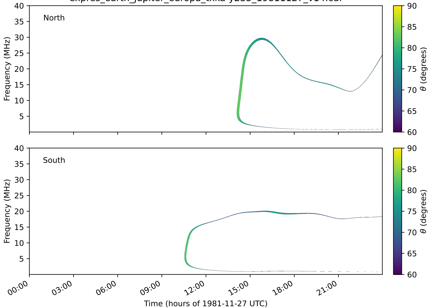
expres_earth_jupiter_europa_txka-y235_19811127_v14.cdf
