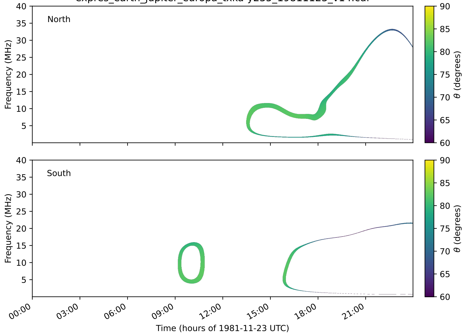
expres_earth_jupiter_europa_txka-y235_19811123_v14.cdf
