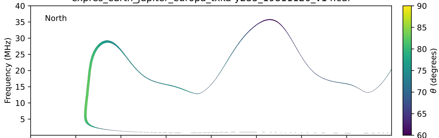
expres_earth_jupiter_europa_txka-y235_19811120_v14.cdf
