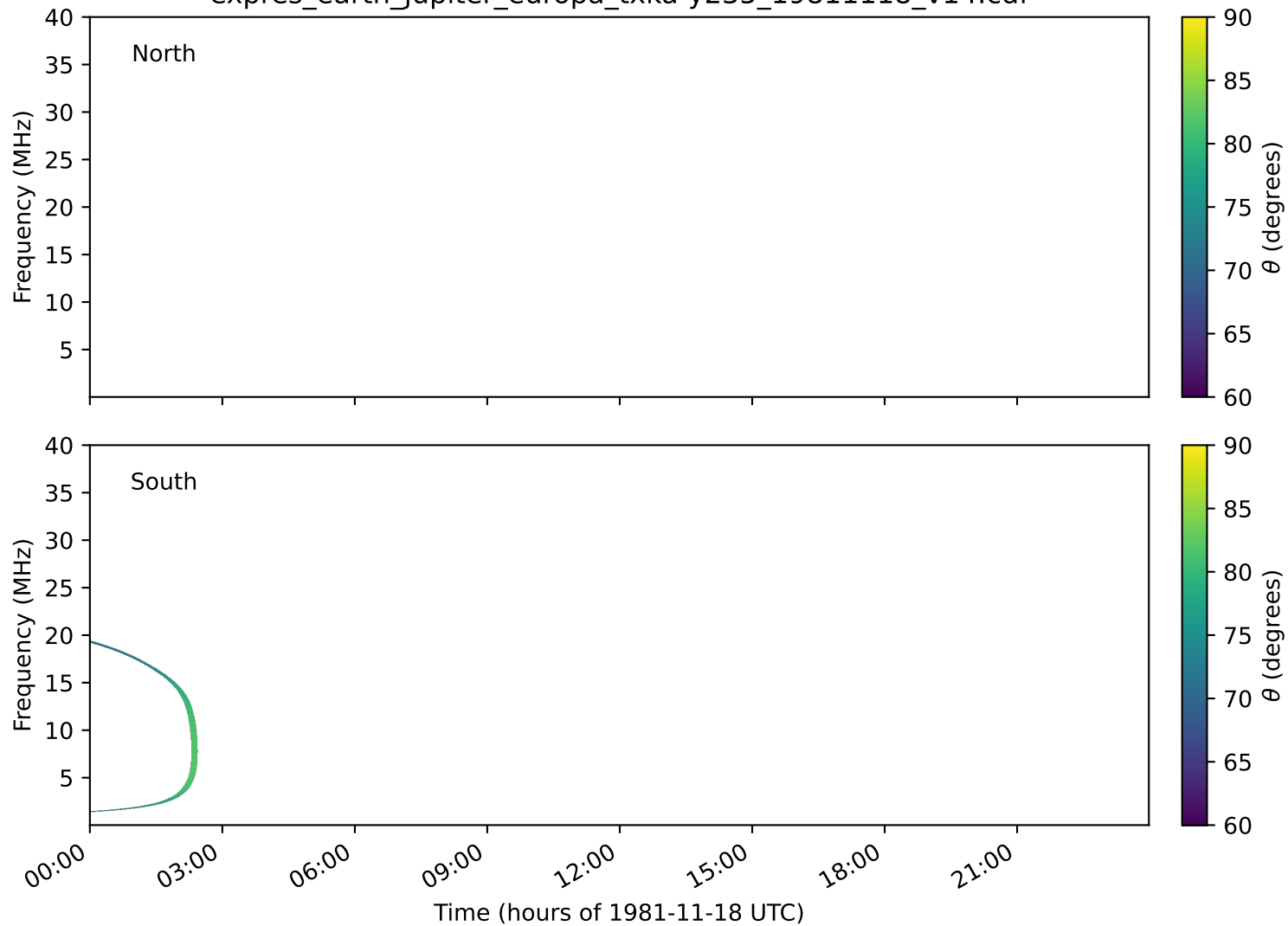
expres_earth_jupiter_europa_txka-y235_19811118_v14.cdf
