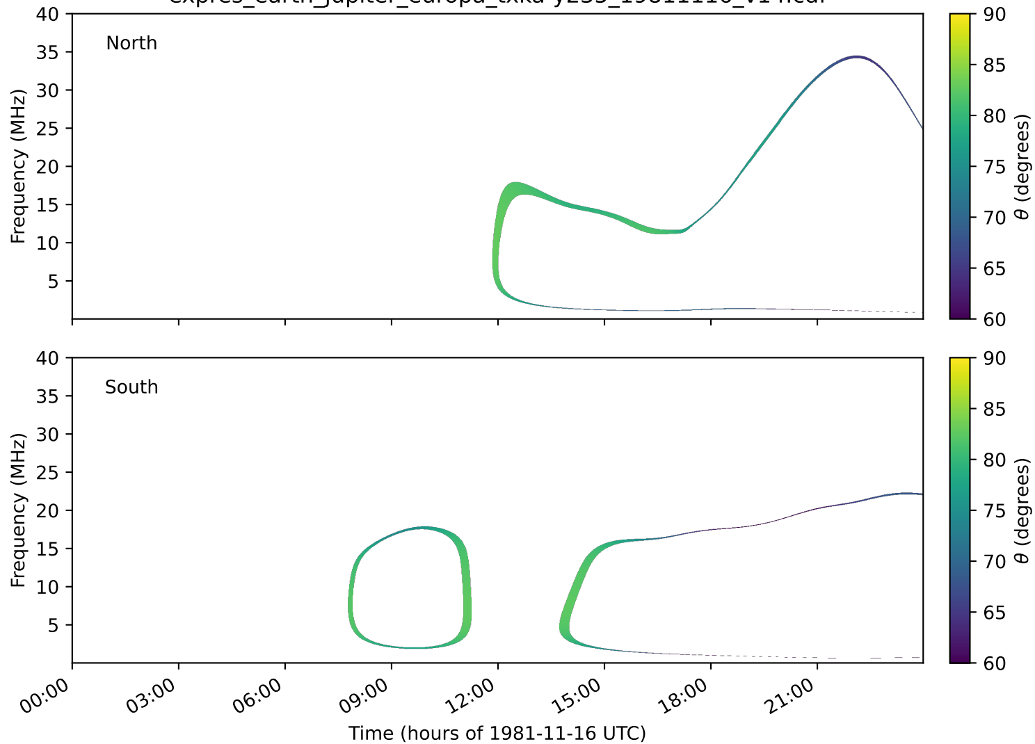
expres_earth_jupiter_europa_txka-y235_19811116_v14.cdf
