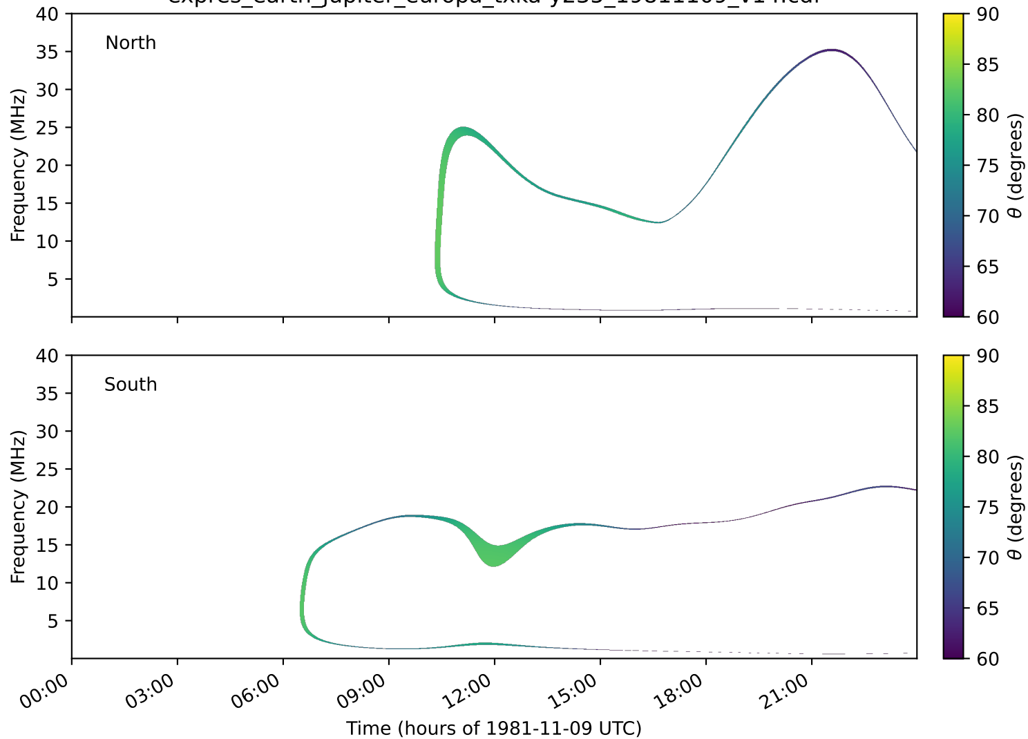
expres_earth_jupiter_europa_txka-y235_19811109_v14.cdf
