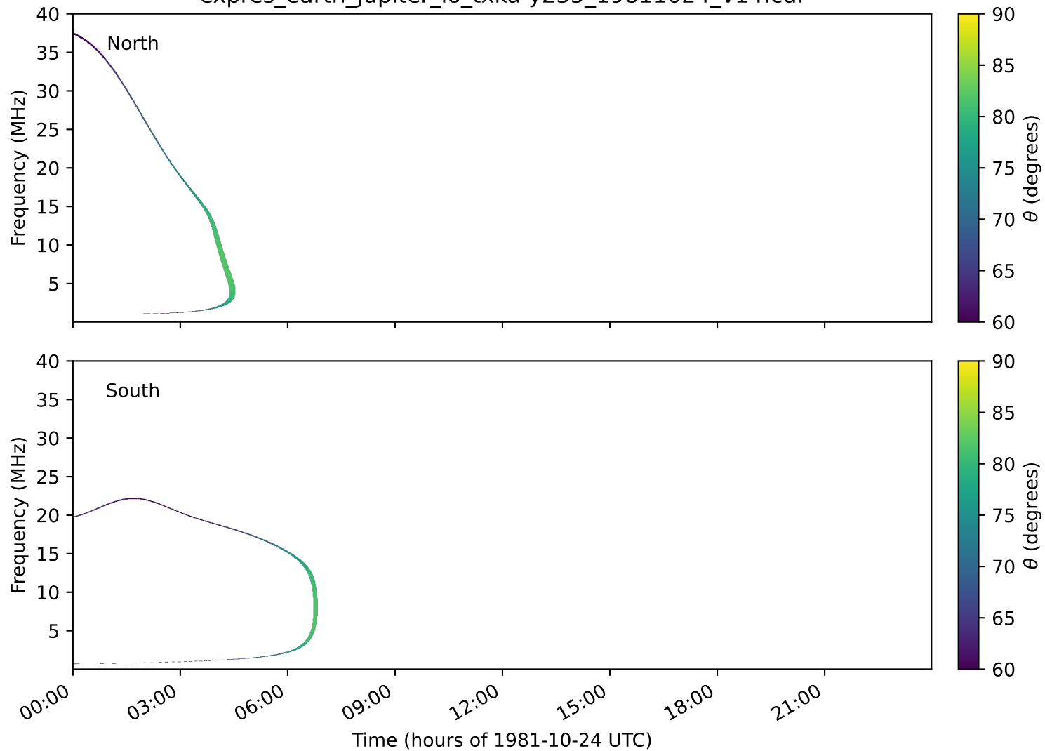
expres_earth_jupiter_io_txka-y235_19811024_v14.cdf
