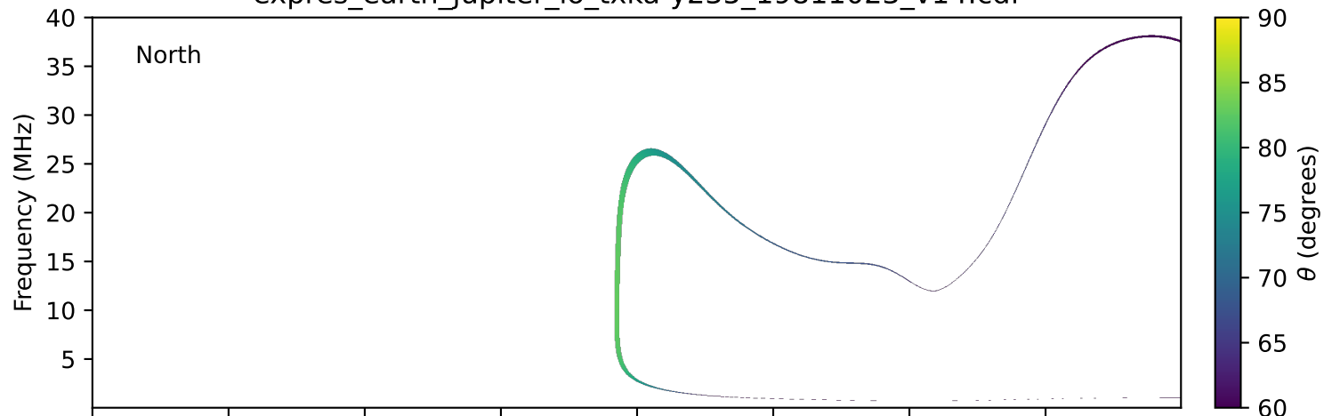
expres_earth_jupiter_io_txka-y235_19811023_v14.cdf
