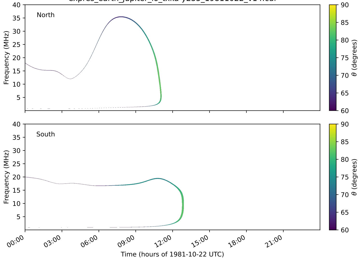
expres_earth_jupiter_io_txka-y235_19811022_v14.cdf
