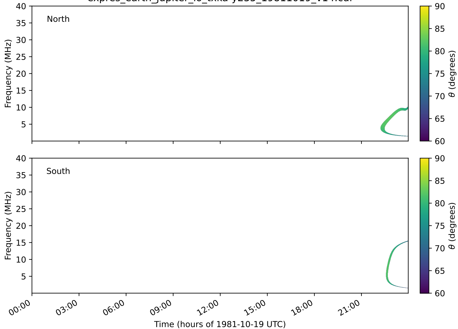
expres_earth_jupiter_io_txka-y235_19811019_v14.cdf
