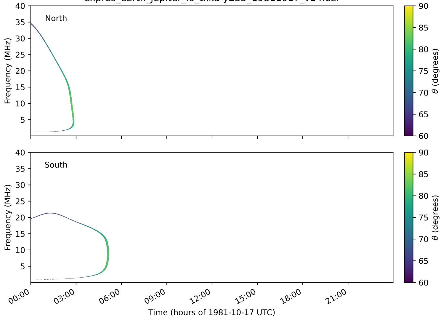
expres_earth_jupiter_io_txka-y235_19811017_v14.cdf
