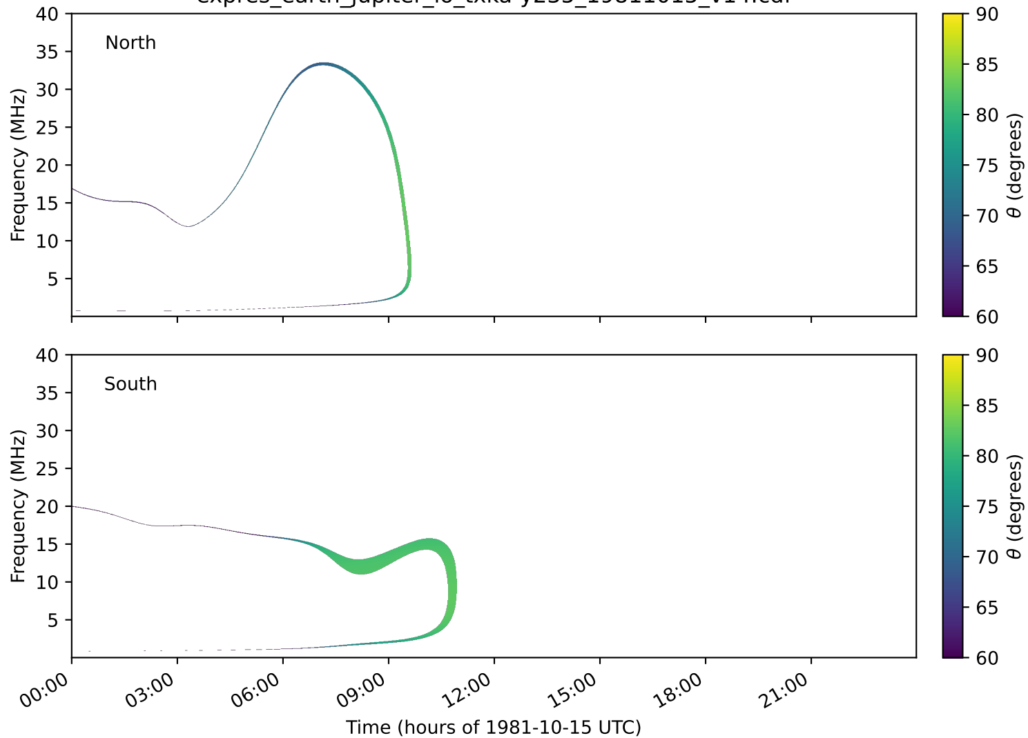
expres_earth_jupiter_io_txka-y235_19811015_v14.cdf
