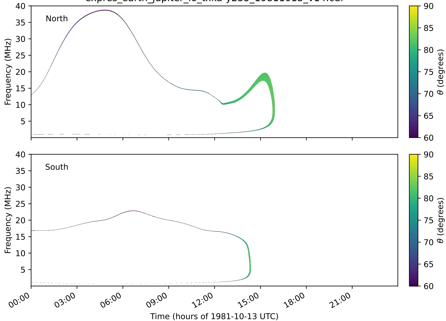
expres_earth_jupiter_io_txka-y235_19811013_v14.cdf
