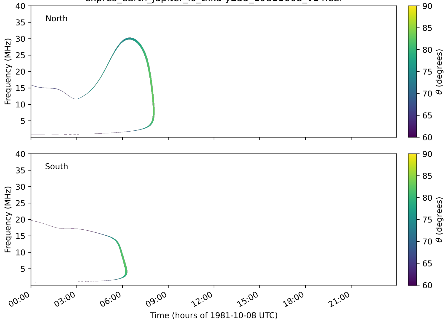
expres_earth_jupiter_io_txka-y235_19811008_v14.cdf
