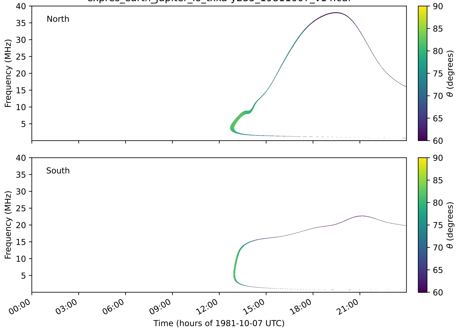
expres_earth_jupiter_io_txka-y235_19811007_v14.cdf
