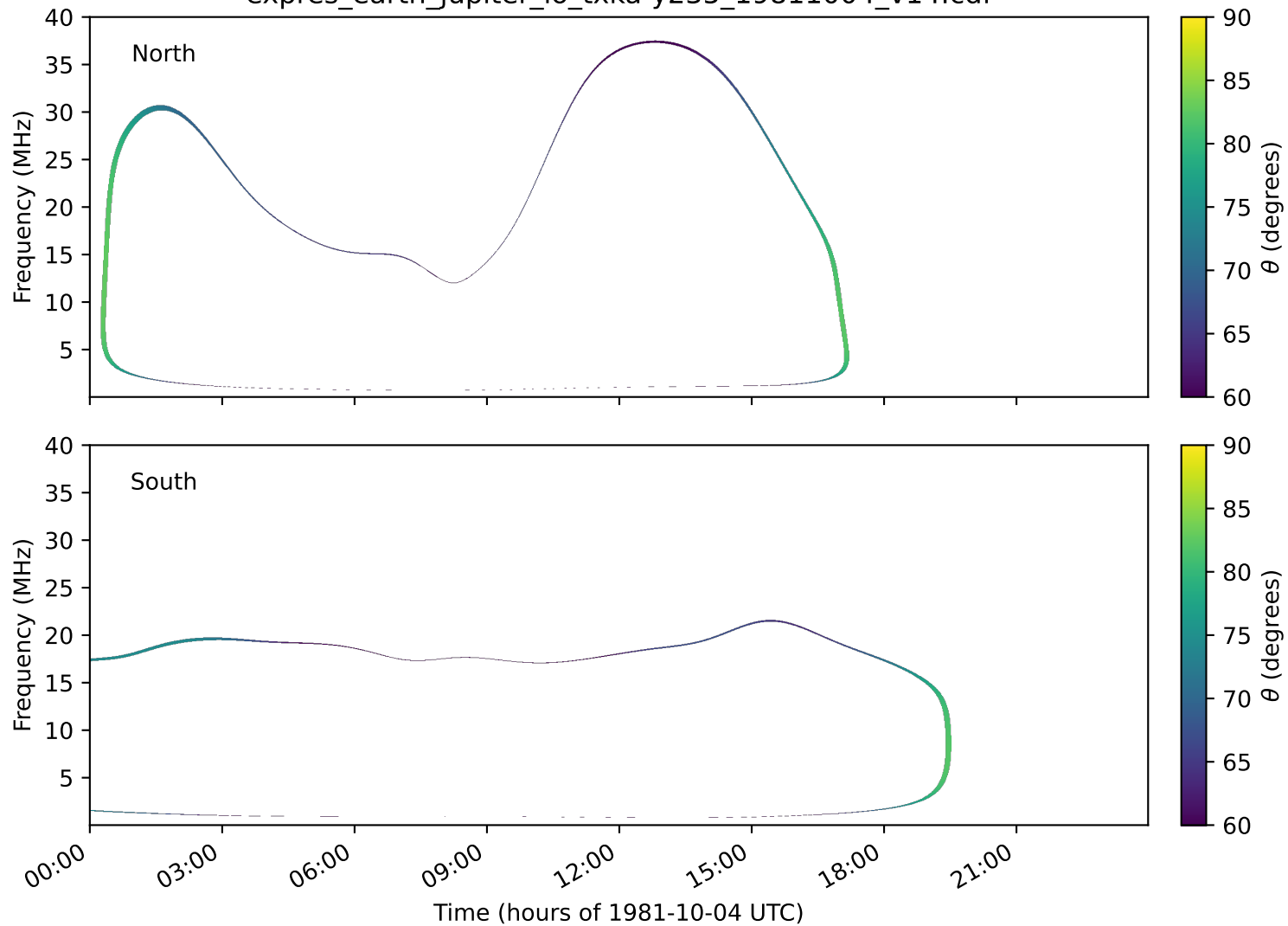
expres_earth_jupiter_io_txka-y235_19811004_v14.cdf
