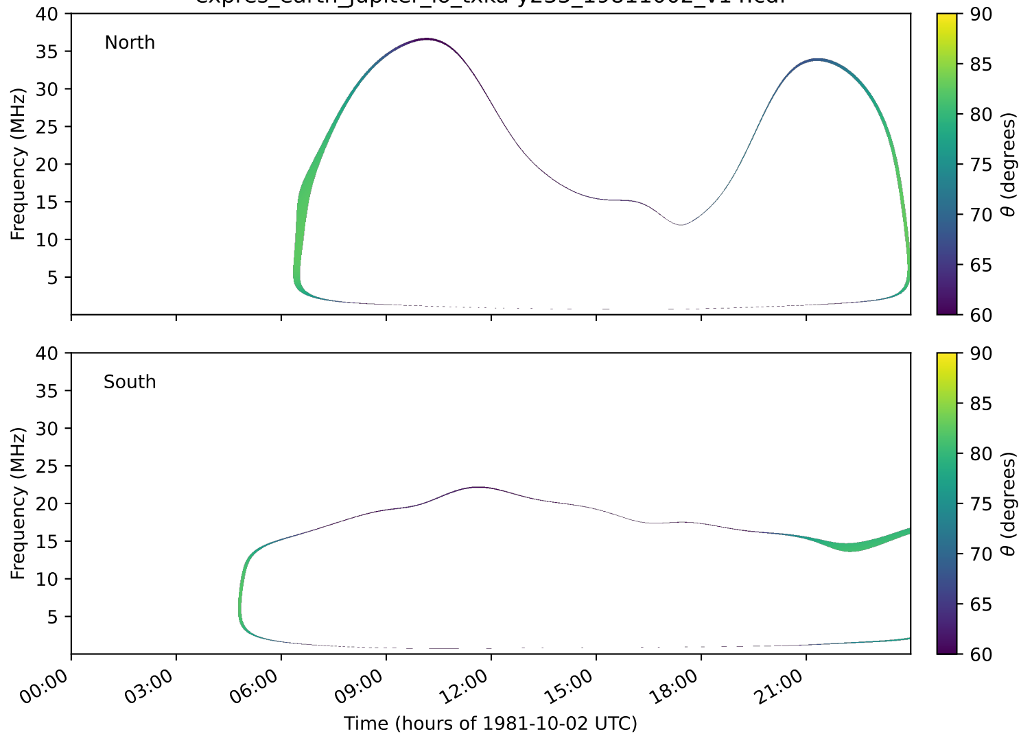
expres_earth_jupiter_io_txka-y235_19811002_v14.cdf
