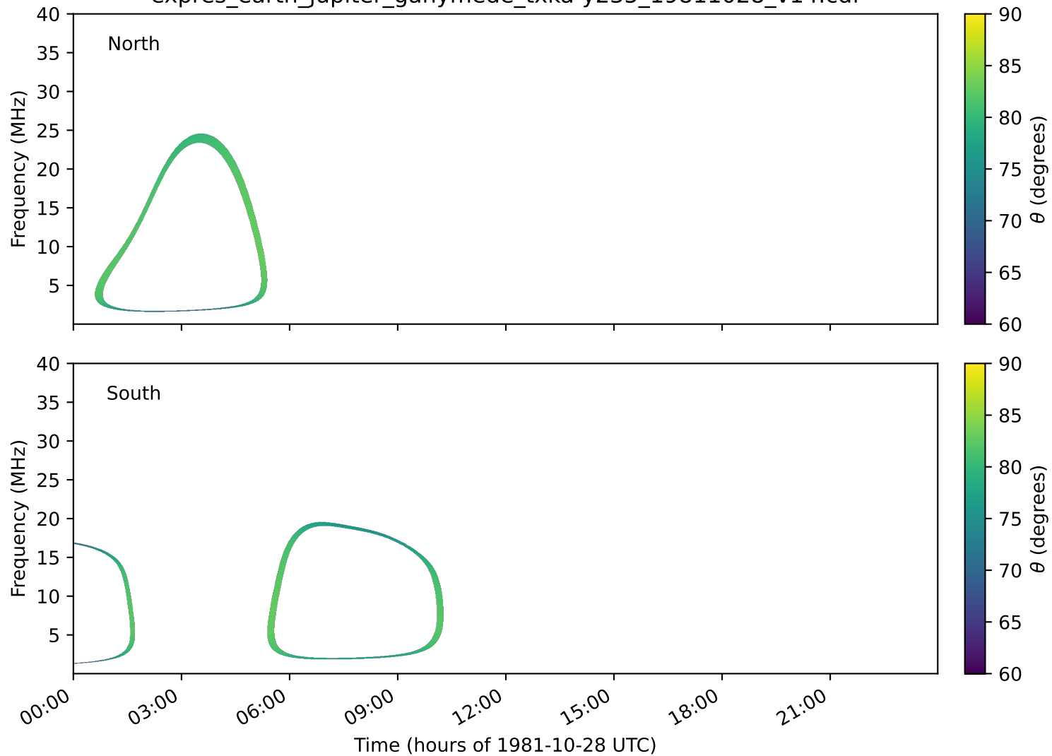
expres_earth_jupiter_ganymede_txka-y235_19811028_v14.cdf
