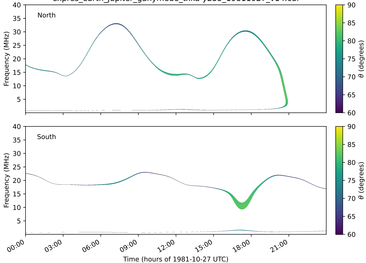
expres_earth_jupiter_ganymede_txka-y235_19811027_v14.cdf
