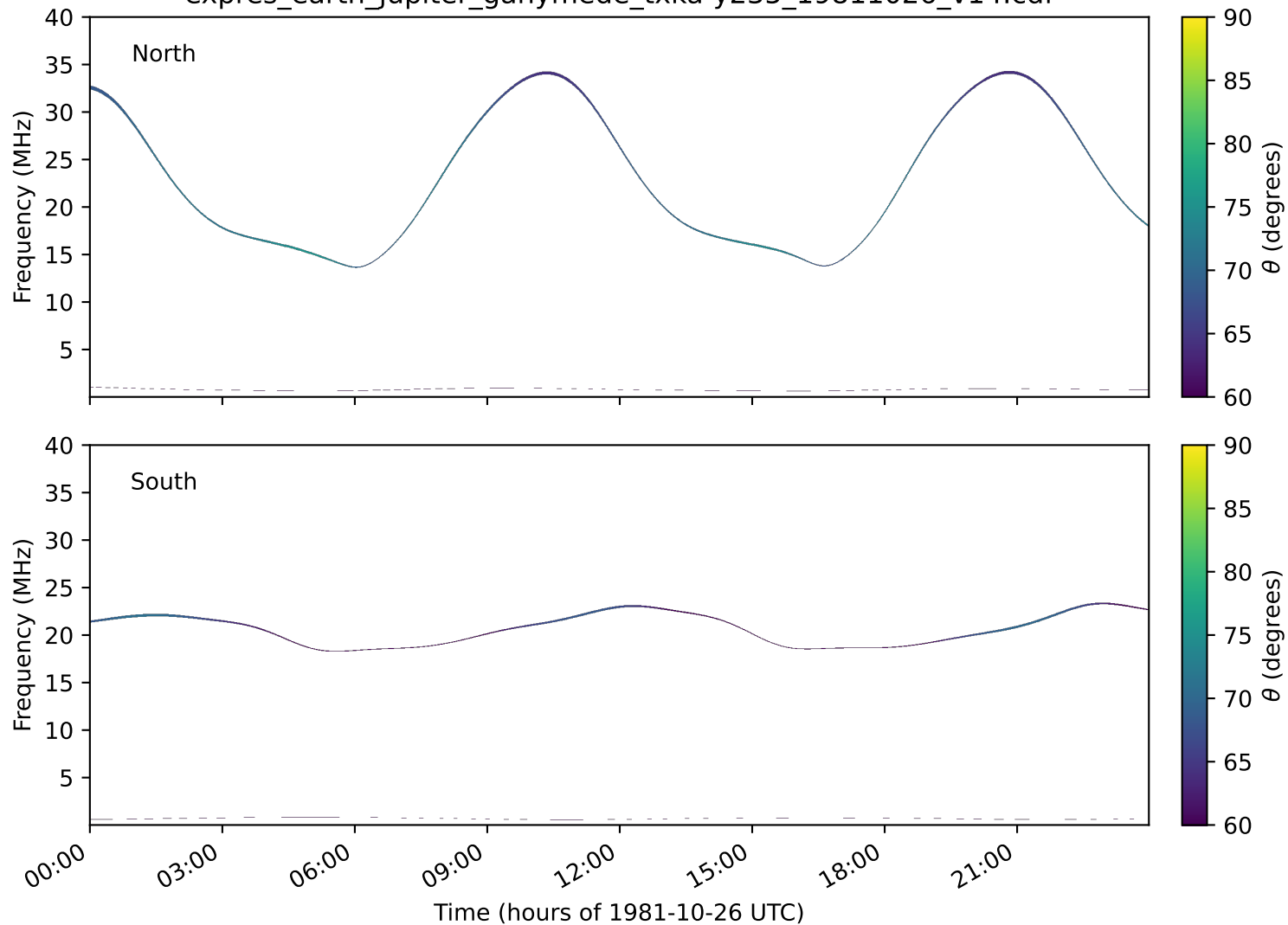
expres_earth_jupiter_ganymede_txka-y235_19811026_v14.cdf
