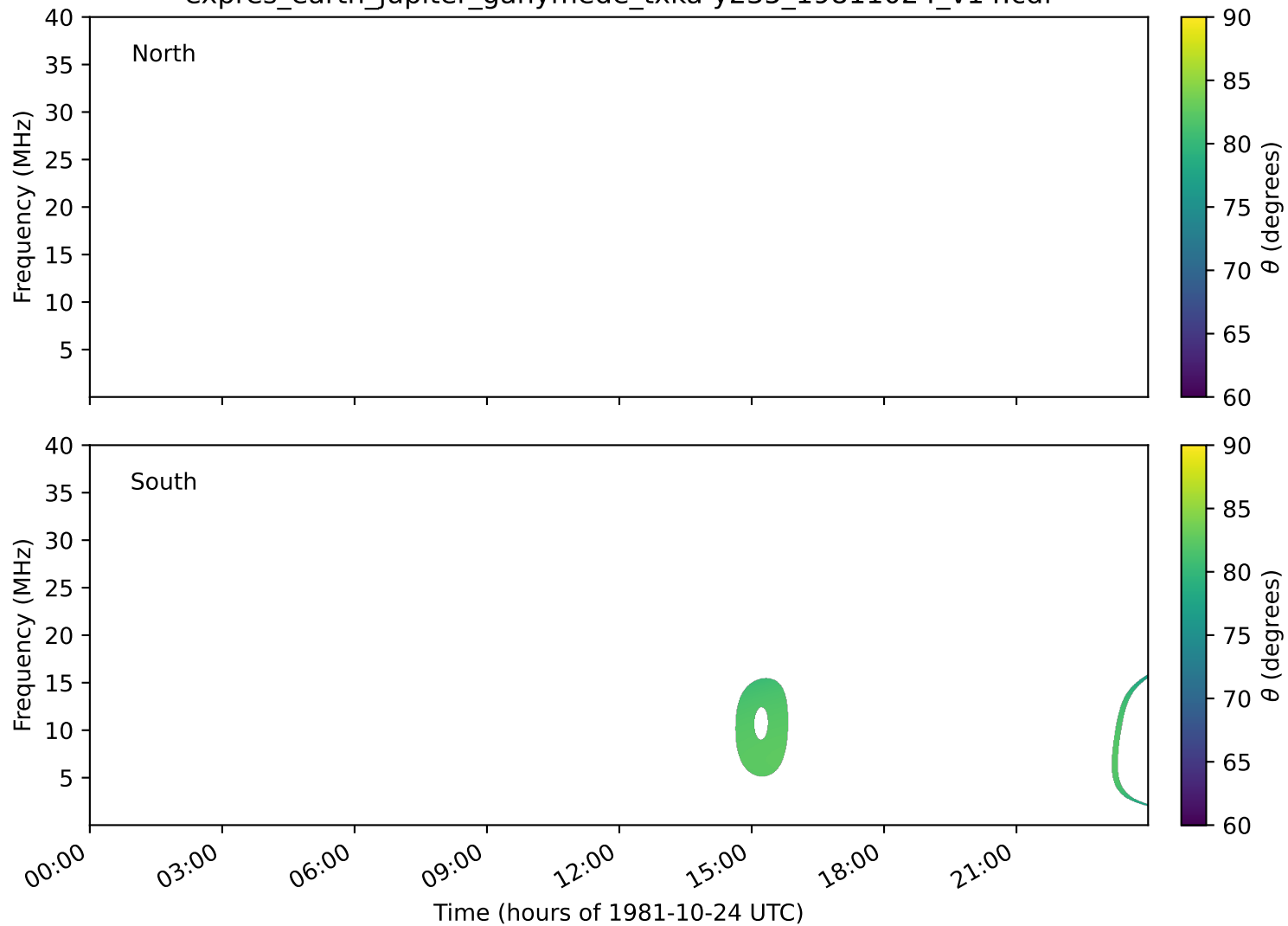
expres_earth_jupiter_ganymede_txka-y235_19811024_v14.cdf
