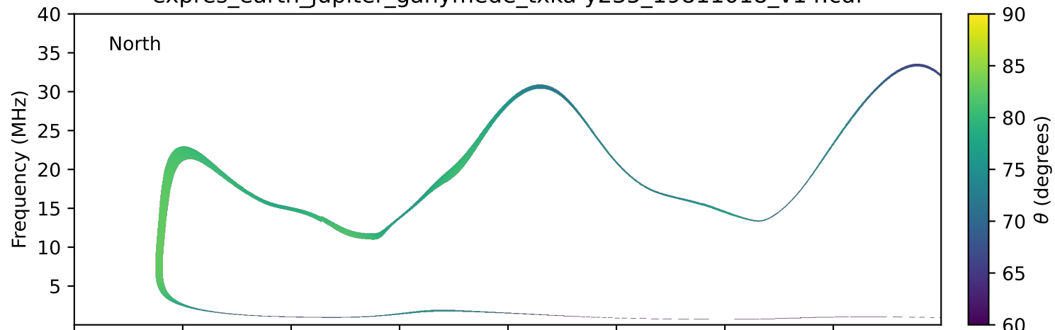
expres_earth_jupiter_ganymede_txka-y235_19811018_v14.cdf
