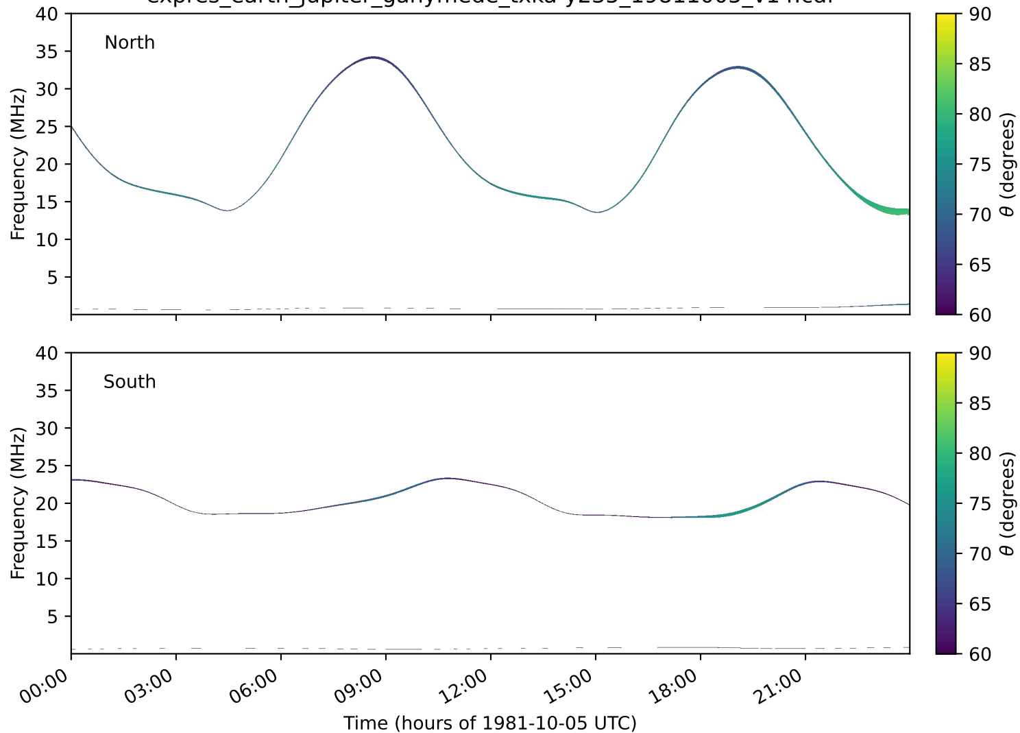
expres_earth_jupiter_ganymede_txka-y235_19811005_v14.cdf
