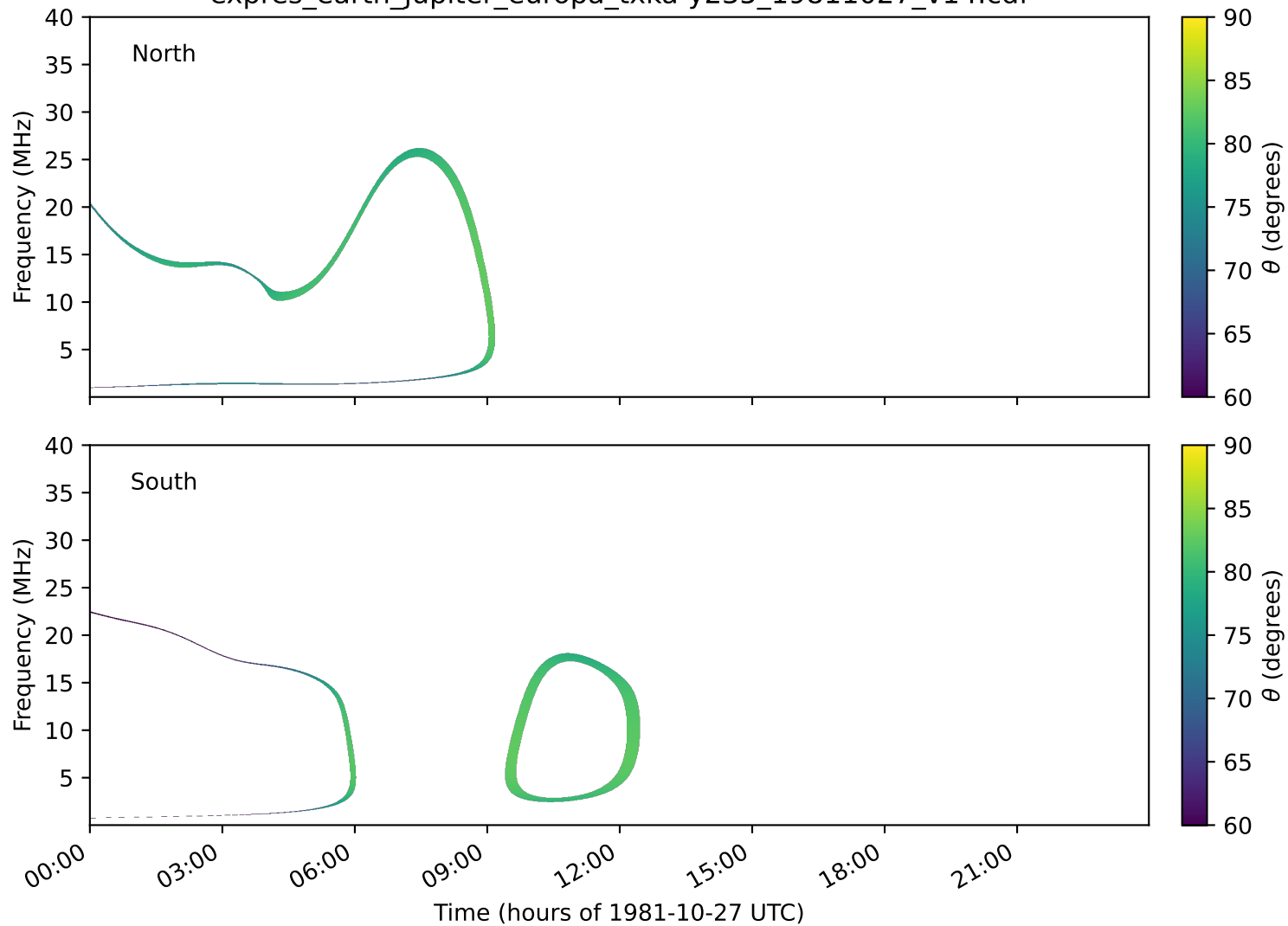
expres_earth_jupiter_europa_txka-y235_19811027_v14.cdf
