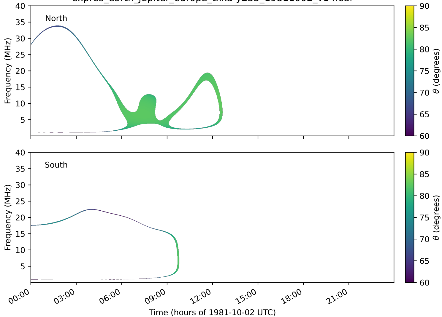
expres_earth_jupiter_europa_txka-y235_19811002_v14.cdf
