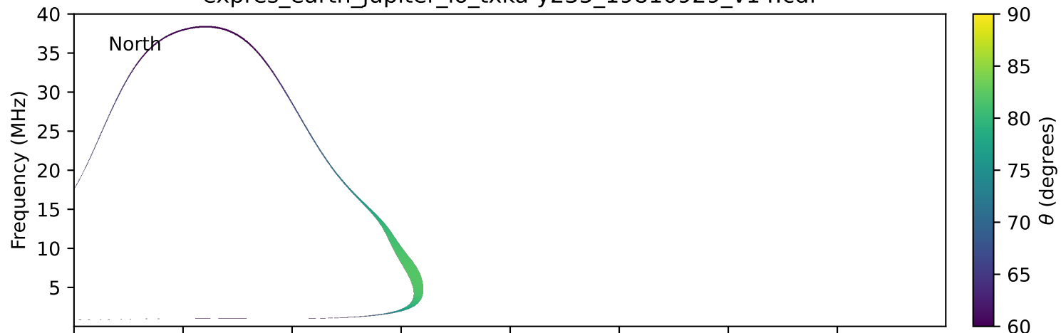
expres_earth_jupiter_io_txka-y235_19810929_v14.cdf
