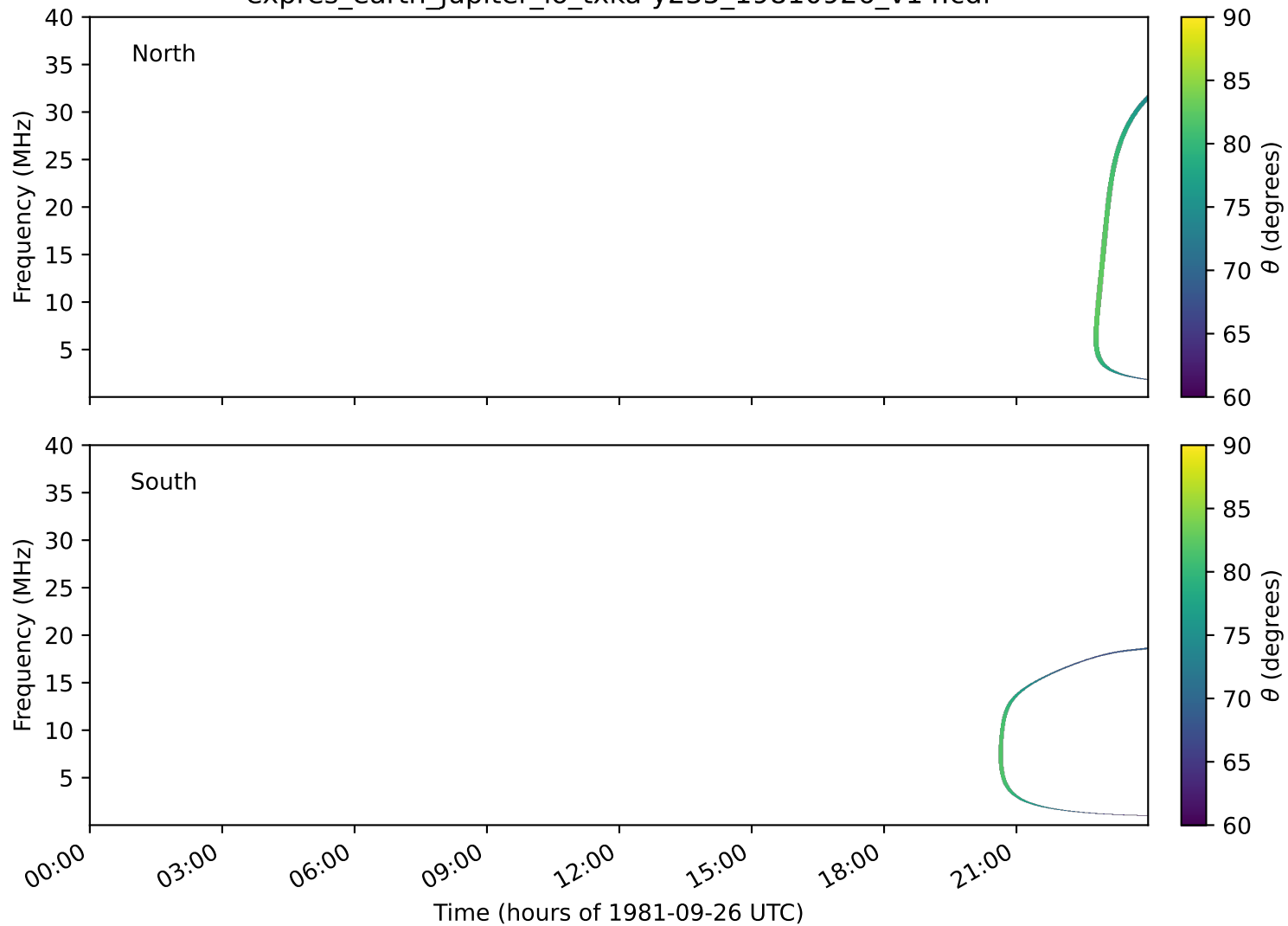
expres_earth_jupiter_io_txka-y235_19810926_v14.cdf
