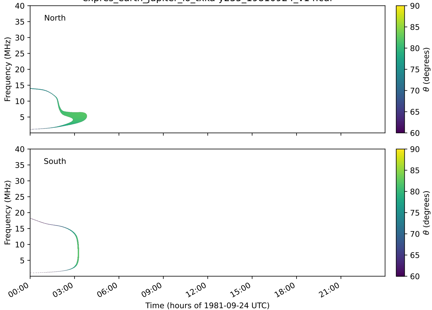
expres_earth_jupiter_io_txka-y235_19810924_v14.cdf
