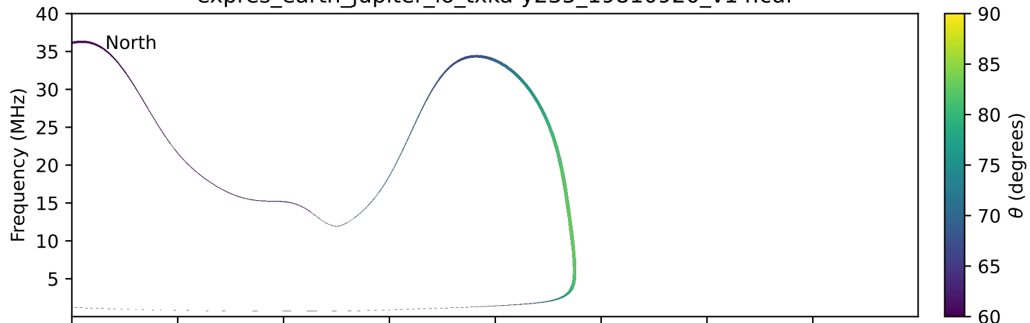
expres_earth_jupiter_io_txka-y235_19810920_v14.cdf
