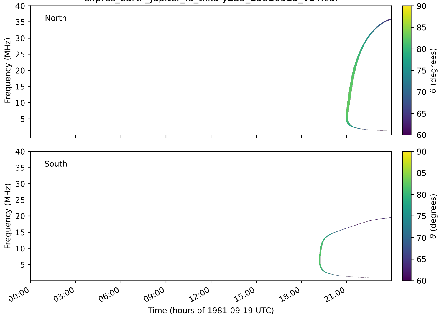
expres_earth_jupiter_io_txka-y235_19810919_v14.cdf
