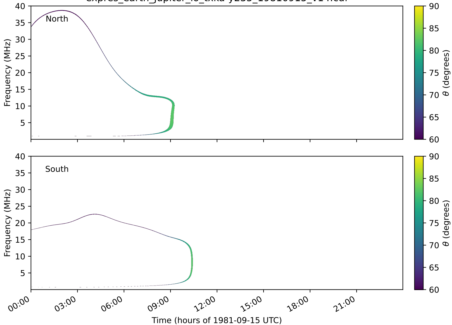
expres_earth_jupiter_io_txka-y235_19810915_v14.cdf
