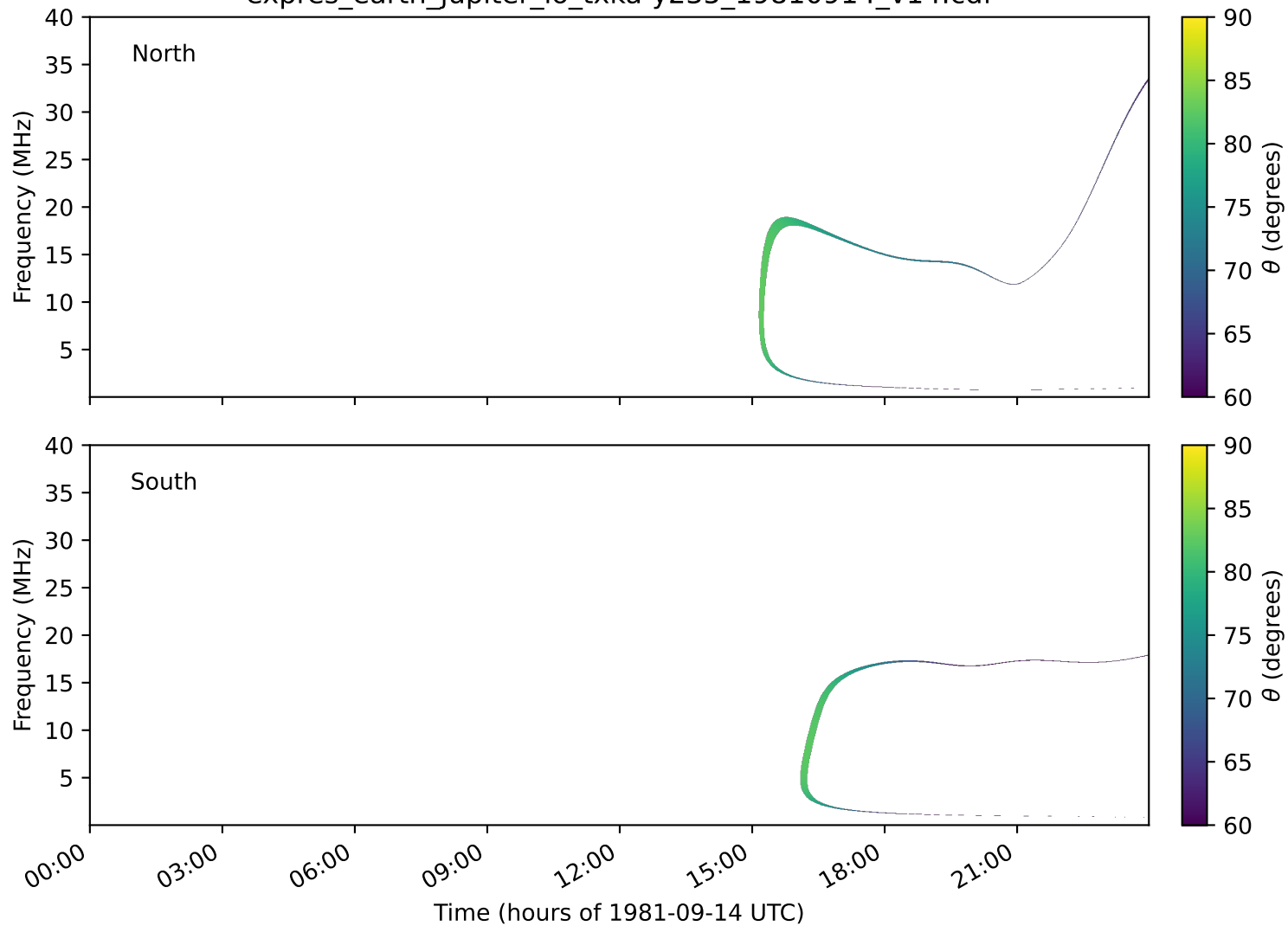
expres_earth_jupiter_io_txka-y235_19810914_v14.cdf
