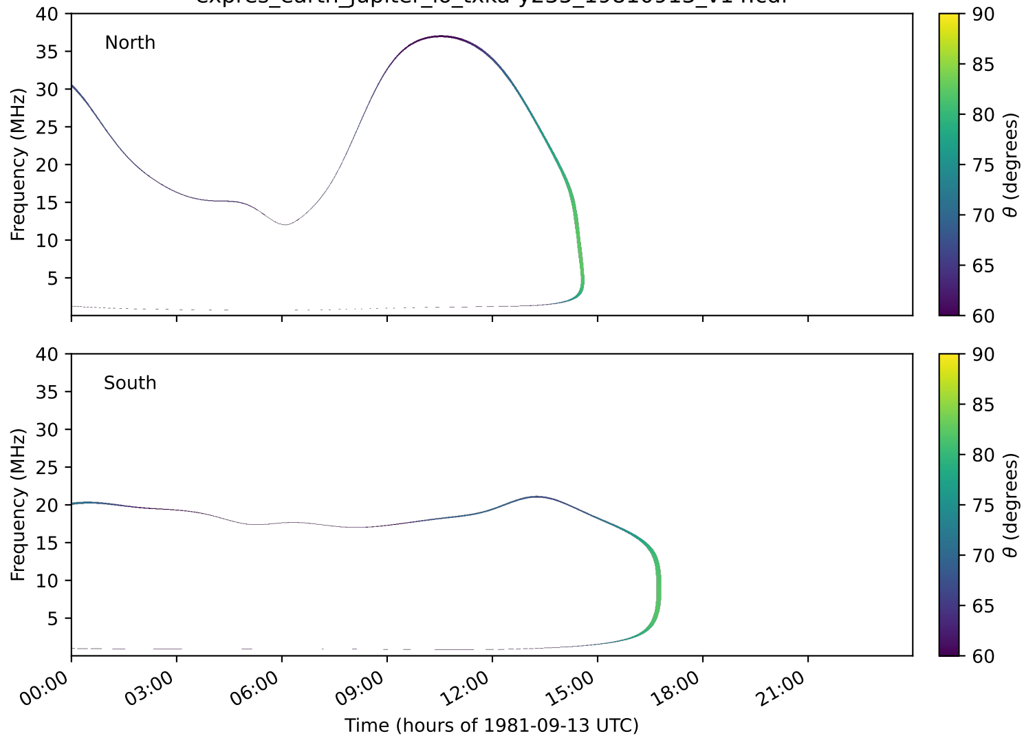
expres_earth_jupiter_io_txka-y235_19810913_v14.cdf
