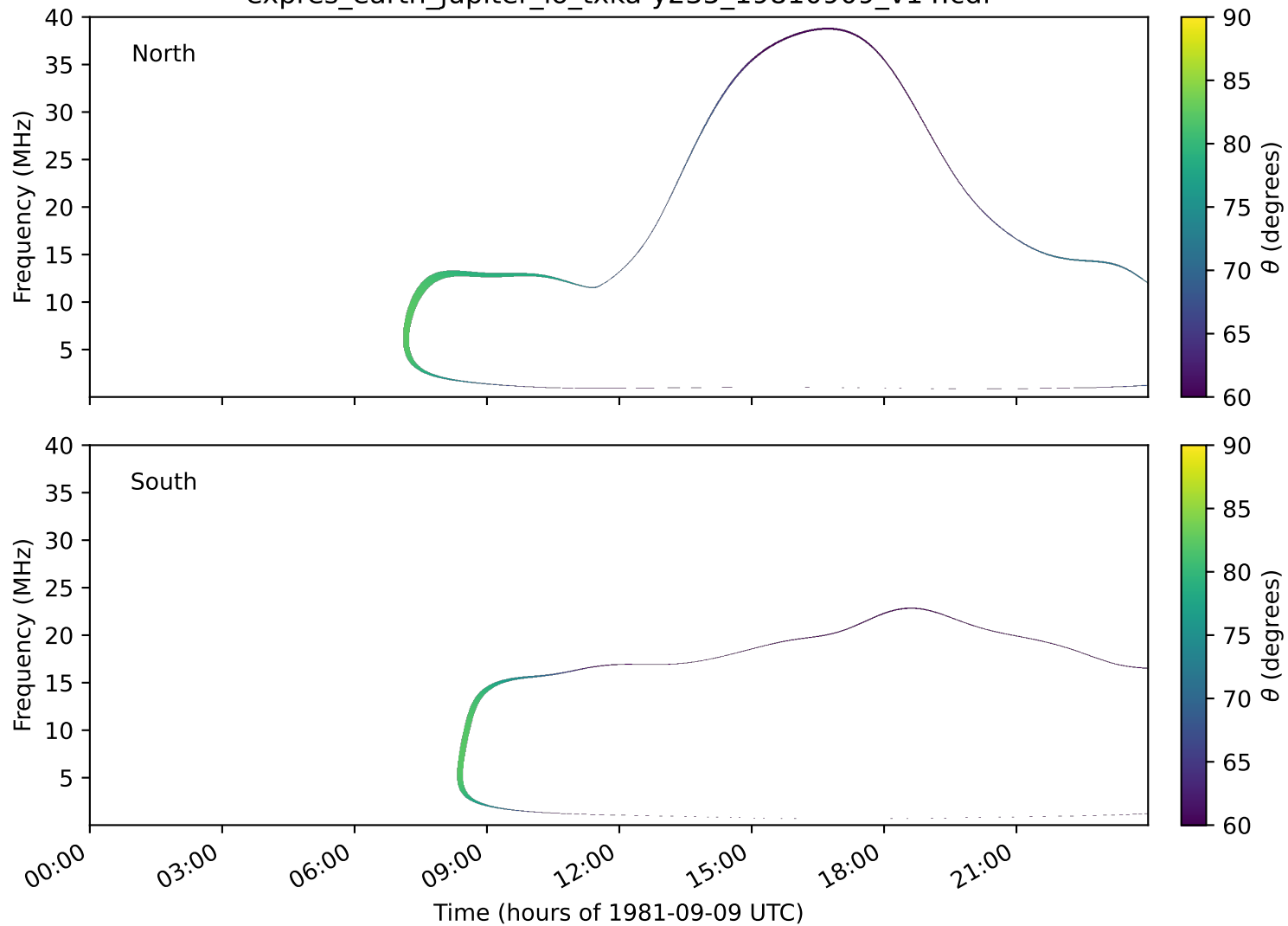
expres_earth_jupiter_io_txka-y235_19810909_v14.cdf
