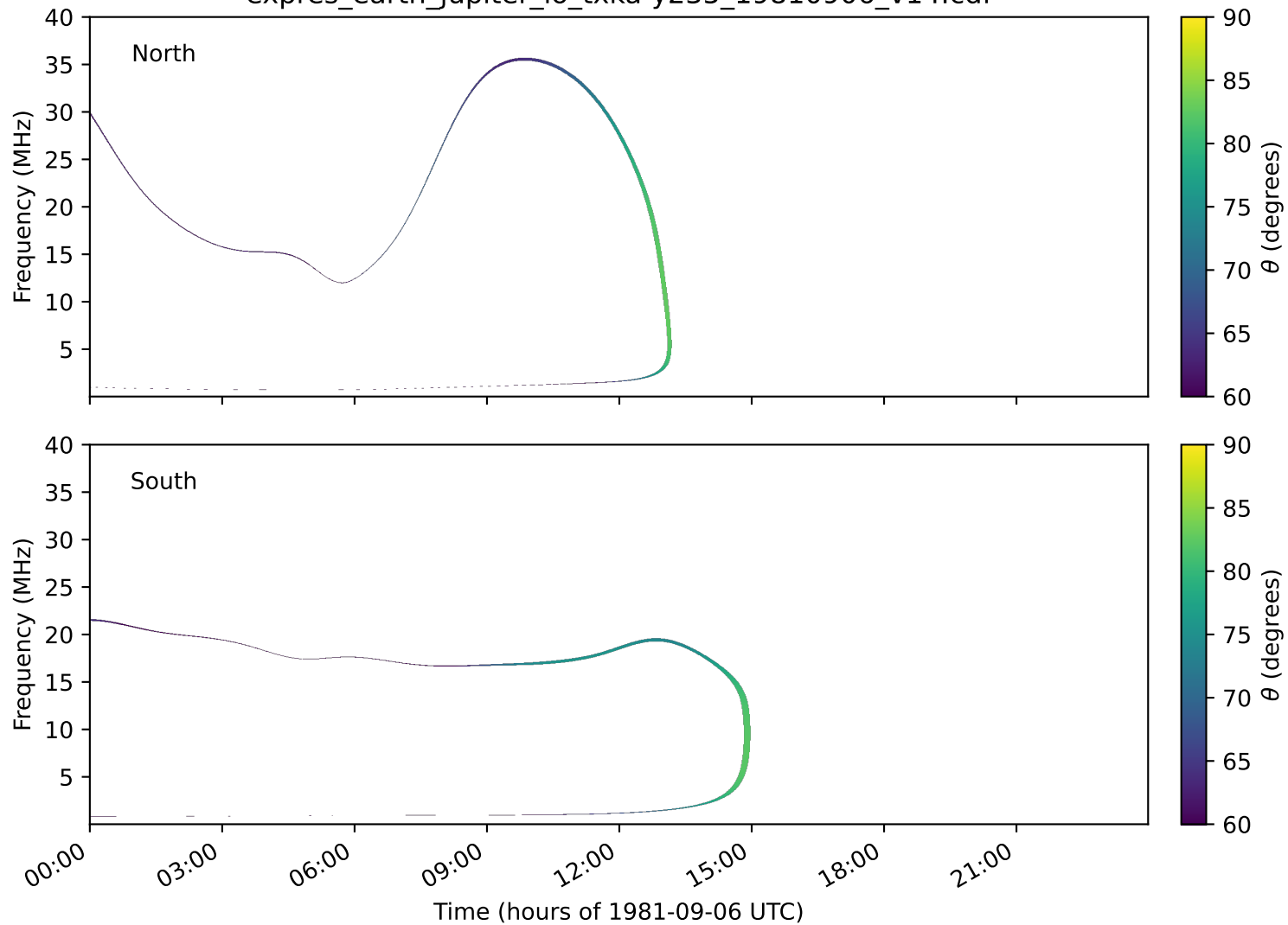
expres_earth_jupiter_io_txka-y235_19810906_v14.cdf
