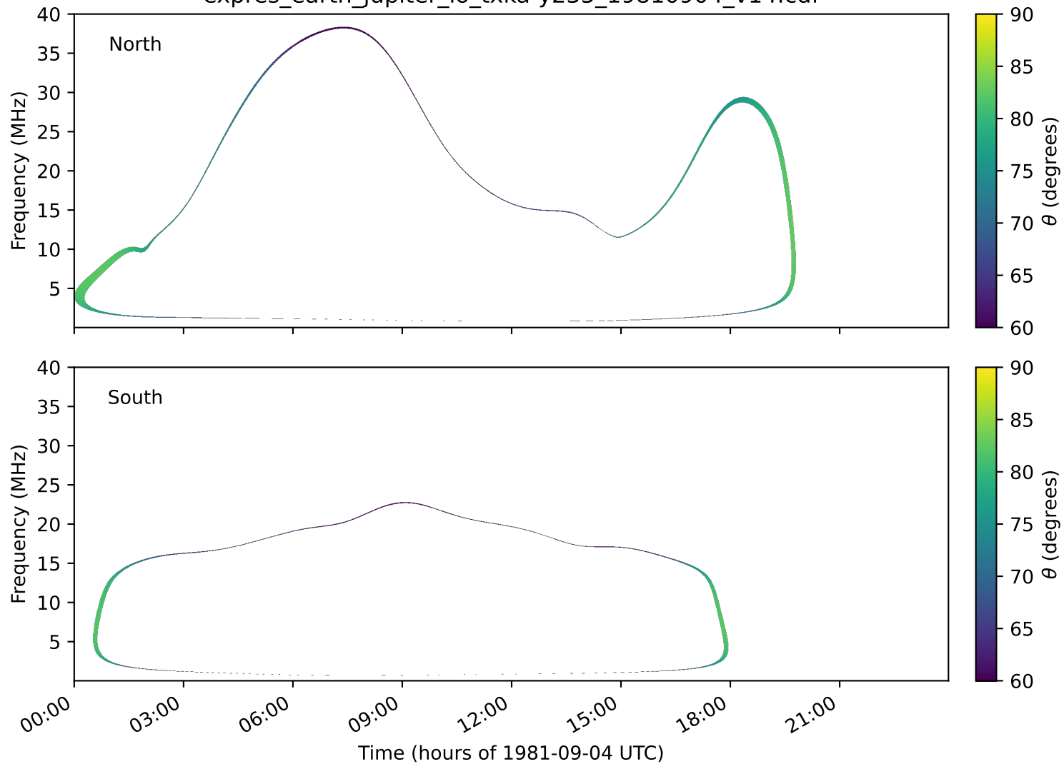
expres_earth_jupiter_io_txka-y235_19810904_v14.cdf
