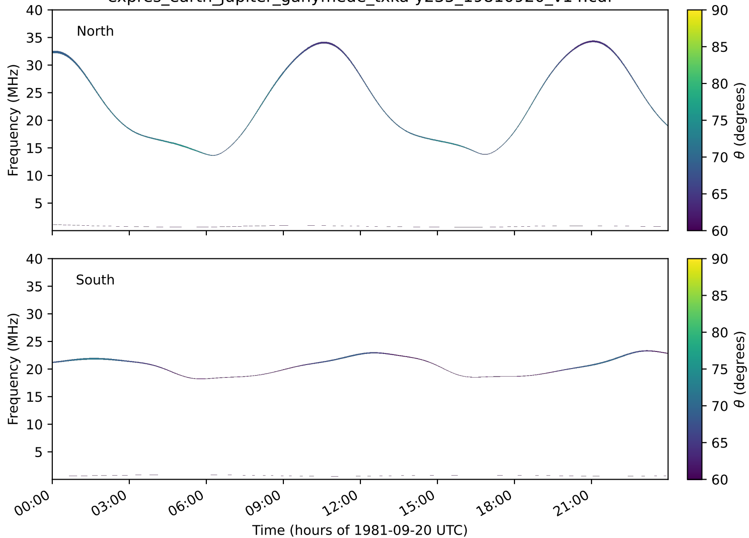
expres_earth_jupiter_ganymede_txka-y235_19810920_v14.cdf
