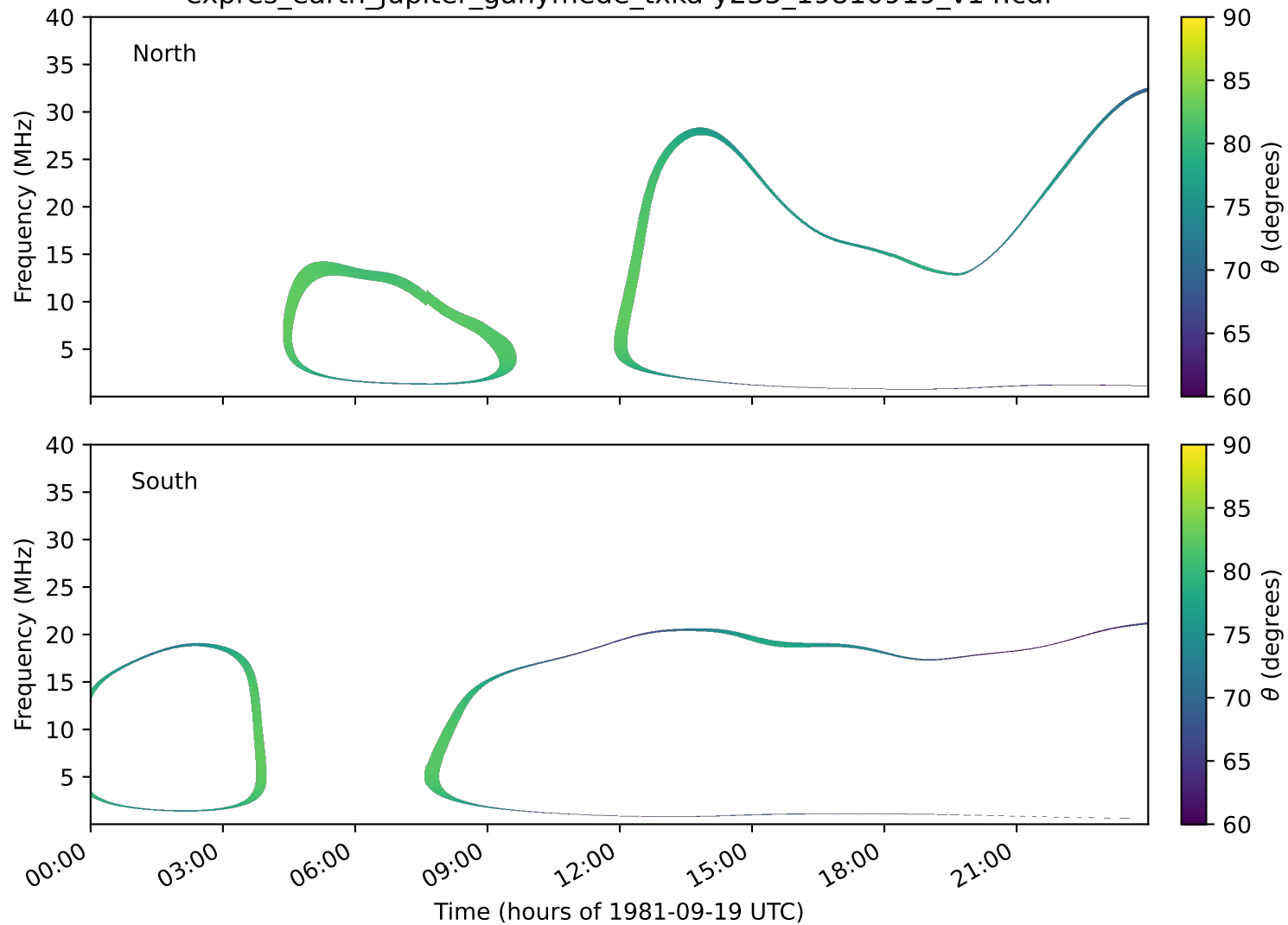
expres_earth_jupiter_ganymede_txka-y235_19810919_v14.cdf
