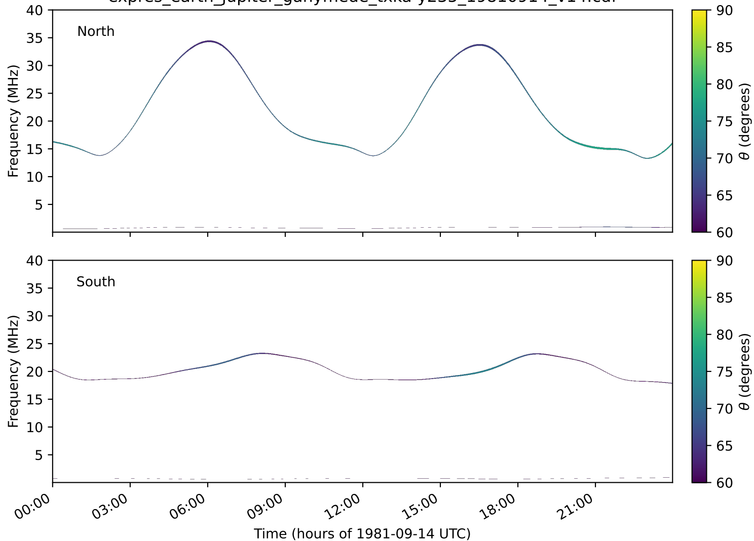
expres_earth_jupiter_ganymede_txka-y235_19810914_v14.cdf
