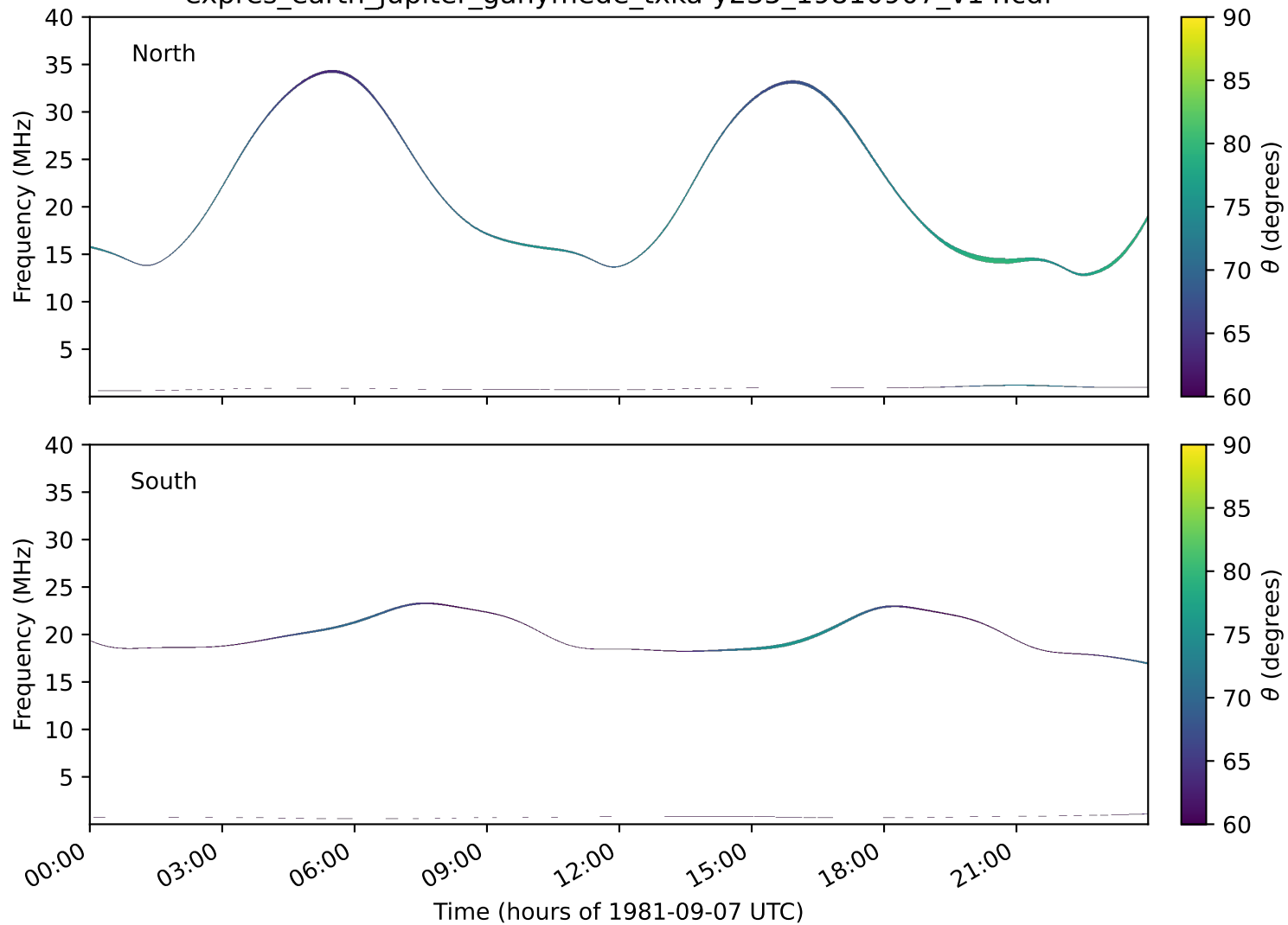
expres_earth_jupiter_ganymede_txka-y235_19810907_v14.cdf
