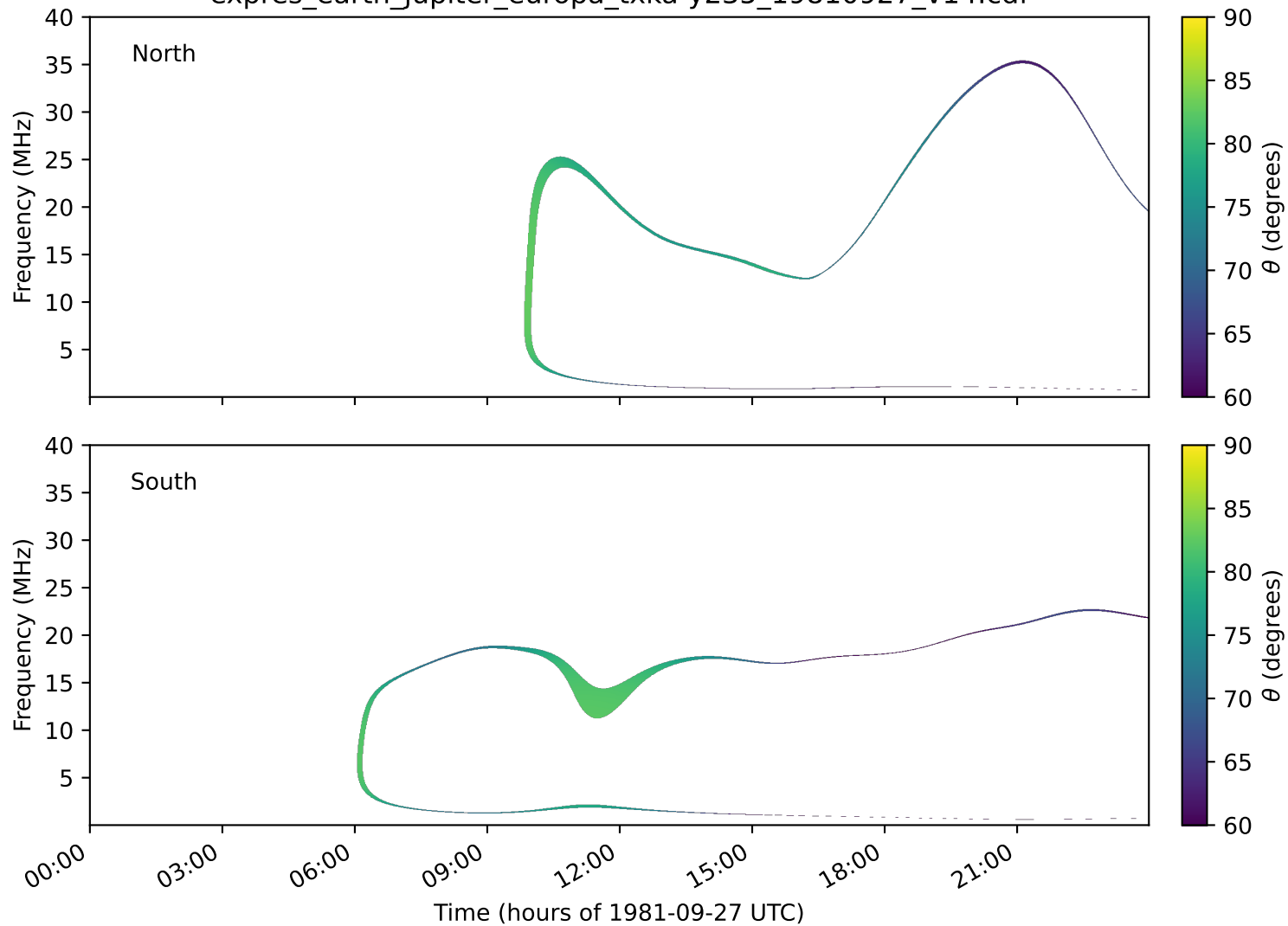
expres_earth_jupiter_europa_txka-y235_19810927_v14.cdf
