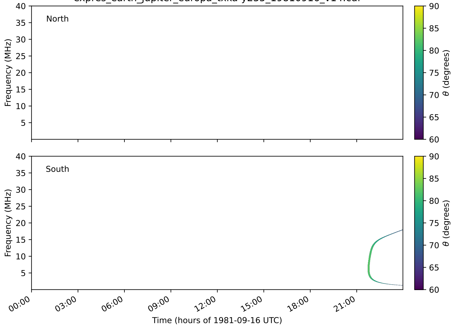
expres_earth_jupiter_europa_txka-y235_19810916_v14.cdf
